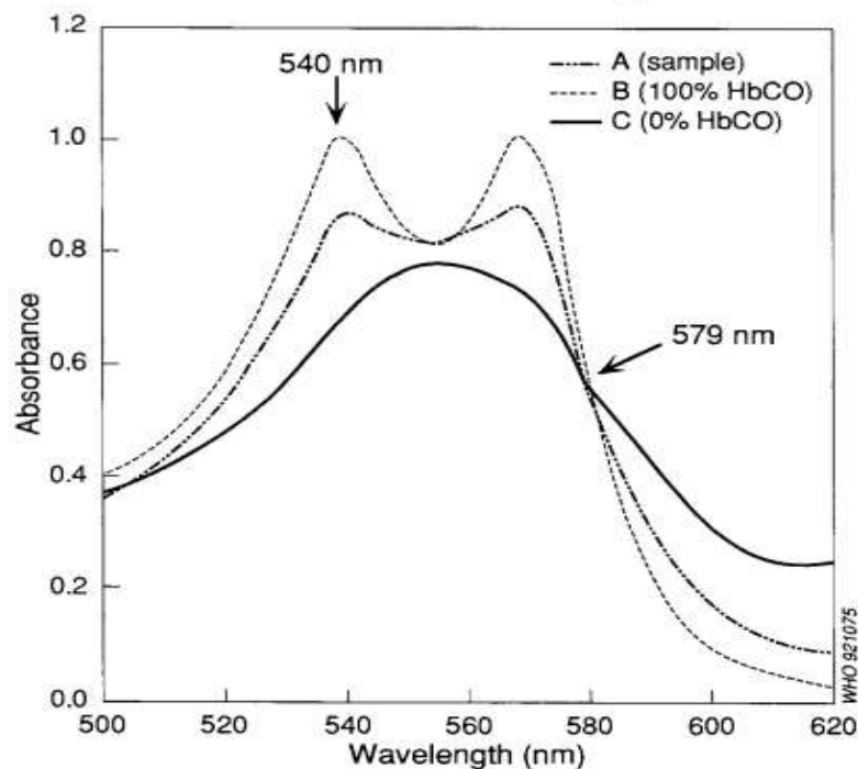
Fig. 11. Spectra obtained using a blood sample from a patient poisoned with carbon monoxide (A), 100% HbCO (B), and 0% HbCO (reduced haemoglobin) (C)
