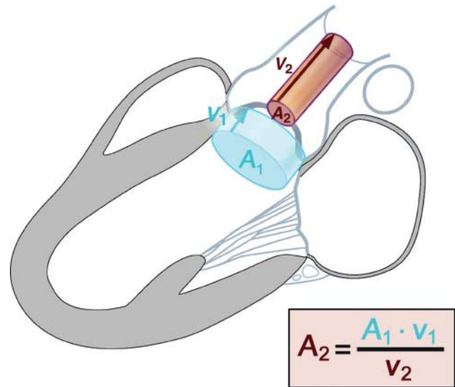
Figure 4 Schematic diagram of continuity equation.
