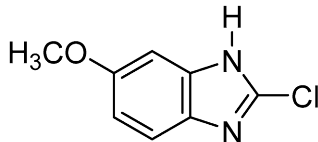
6-methoxy tautomer
