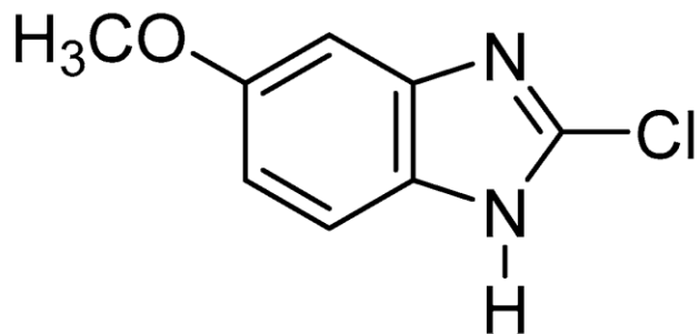
5-methoxy tautomer
